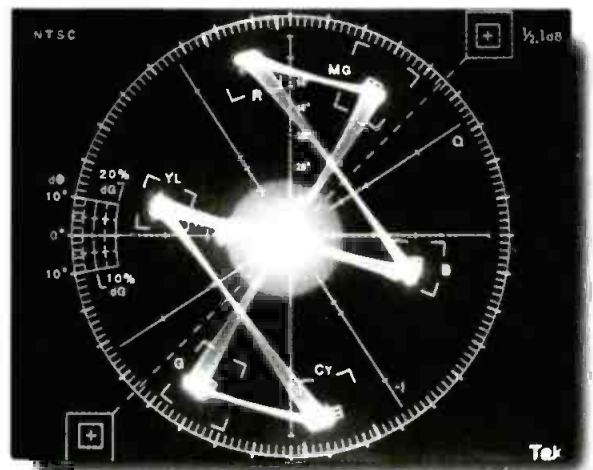
Figure 10. NTSC vectorscope display of a 100/0/100/0 color bars signal derived from a 270Mb/s bit serial digital signal with a 2.092nanosecond p-p, 200Hz timing jitter.
