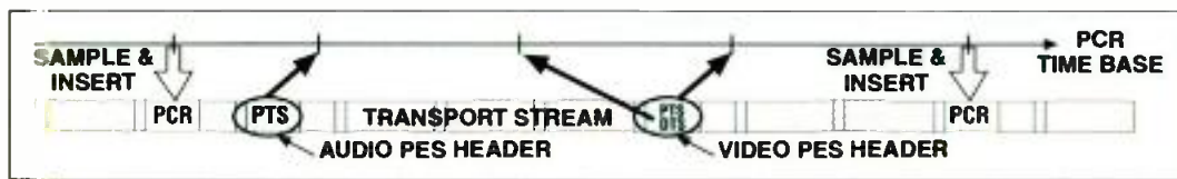
Figure 3. A single-program transport stream showing PCRs and time stamps, essential for timing and synchronization.
