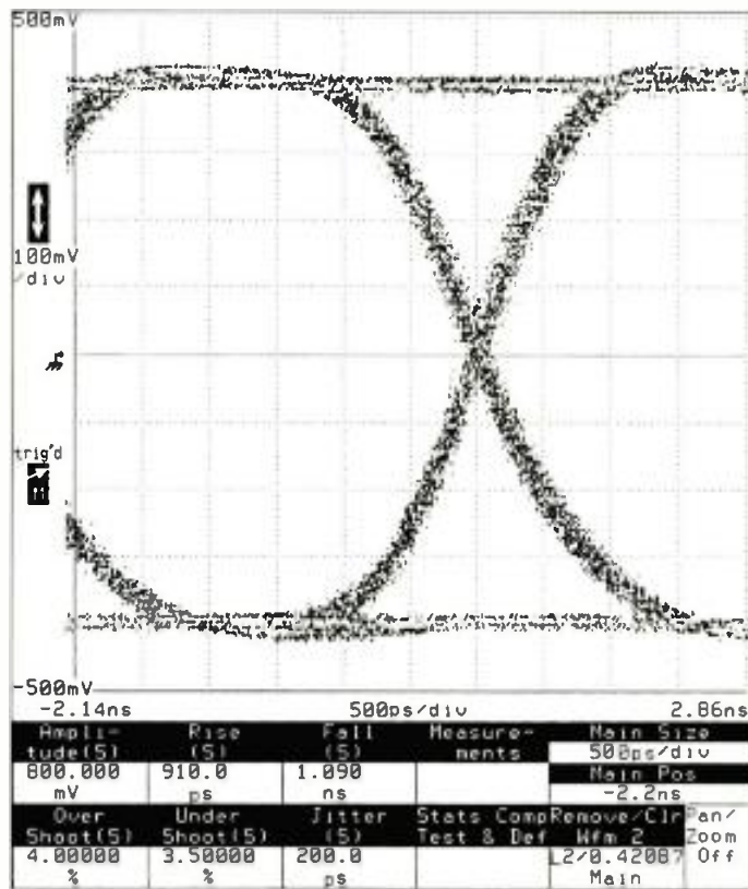
Figure 7. Tektronix 11403 digitizing oscilloscope display printout of a good signal with low jitter. The oscilloscope is triggered by a stable and synchronous reference signal and is programmed to make six performance-indicative measurements. The measured absolute jitter value is 200picoseconds p-p.
